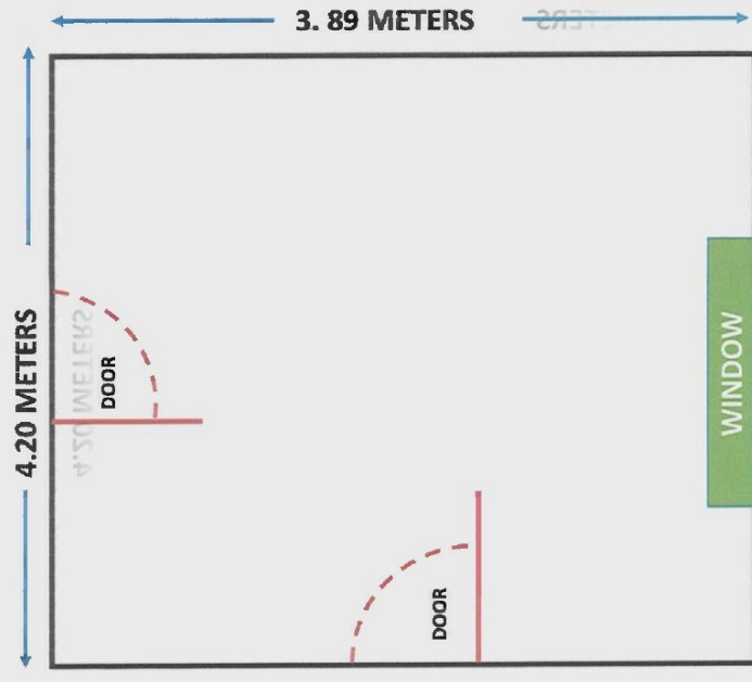
Female Barracks (L-4.20 meters, W-3.89 meters= 16.34 square meters) 2HP
